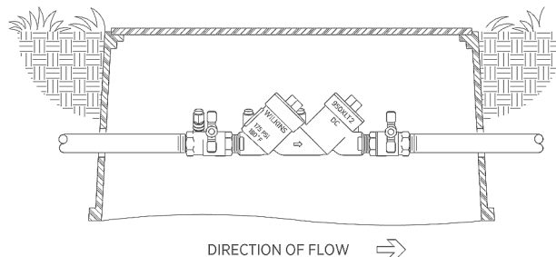
PIT INSTALLATION
