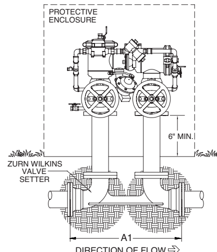
OUTDOOR INSTALLATION
